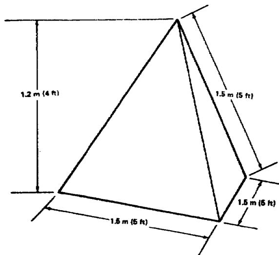
Figure 3-18. Concrete tetrahedron.
